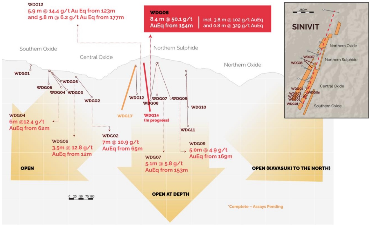
Figure 3 – Long section through the Sinivit target area showing drilling completed to-date with key intervals.
