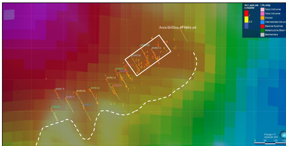
Figure 13: Oblique view of 2024 and historical drilling including Au assays (along drill traces) from Mt Victor, Arau
