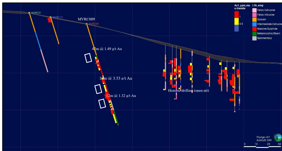
Figure 12: Cross-section through Mt Victor showing Au mineralization intersected in hole MVRC009 relative to historical drilling
