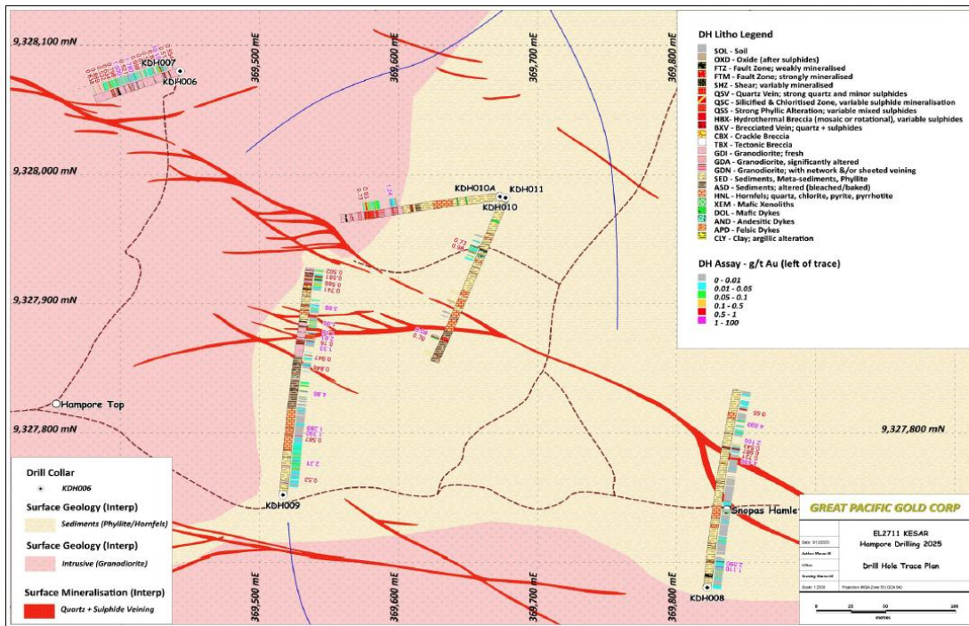
Figure 9 – Geology and structural interpretation of the Hampore target including drill traces and gold assays.
