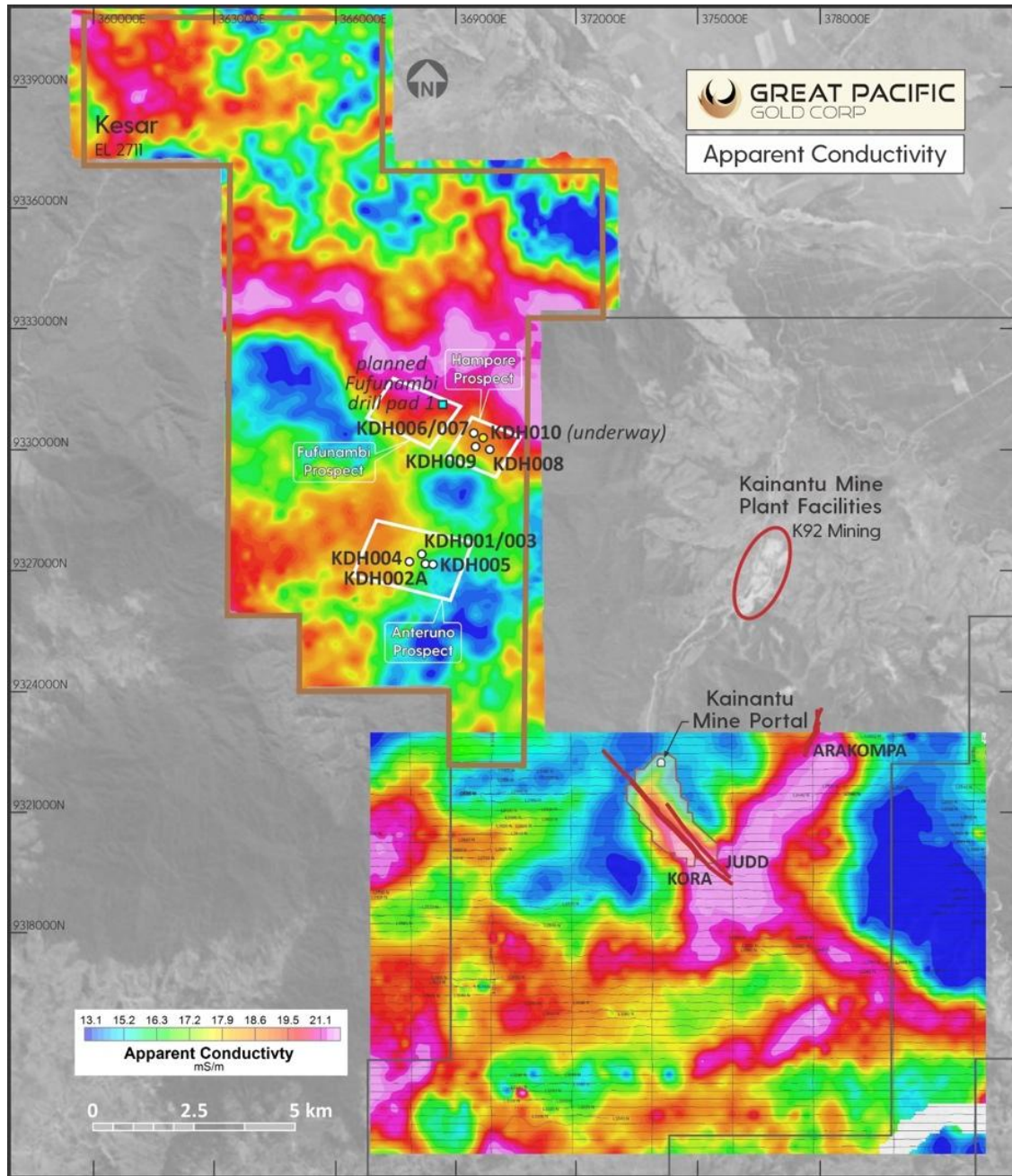
Figure 10 - Kesar Project – MobileMT Survey
