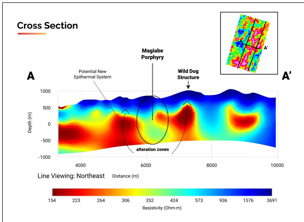
Figure 6: Resistivity cross section highlighting the Magiabe porphyry system, along with the Wild Dog epithermal system. A further epithermal target may be present to the west of Magiabe.
