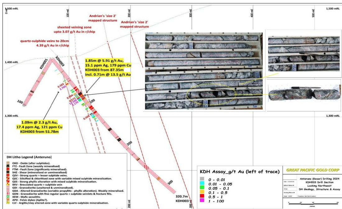
Figure 7 – Drill section of hole KDH003 with downhole lithology and significant gold assays (Anteruno Target).
